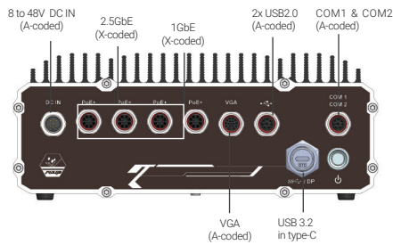
Nuvo-9650AWP
