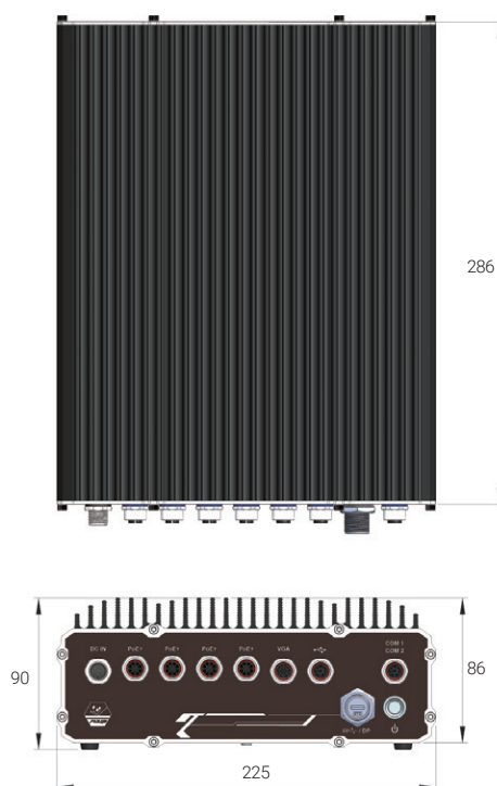
Nuvo-9650AWP
