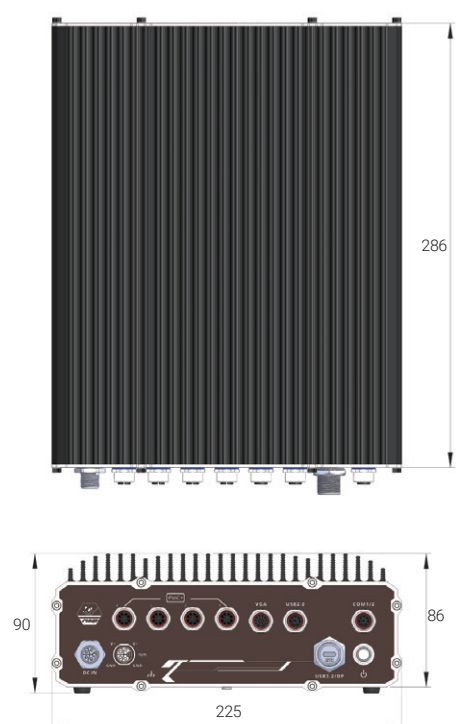
Nuvo-9650AWP-PoE
